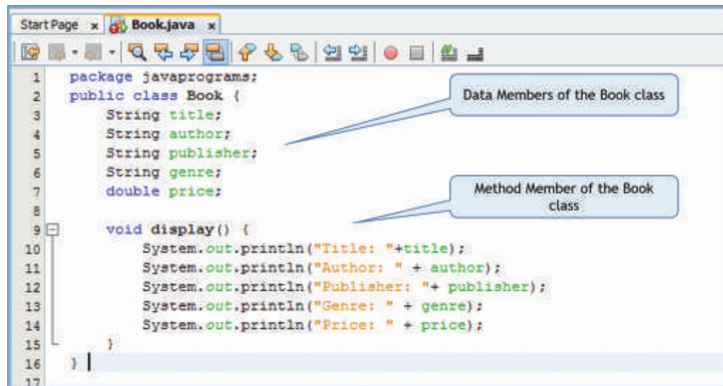
Figure 3.8(a): The Book Class
