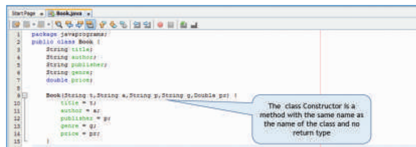
Figure 3.8(b): The Book Class Constructor
