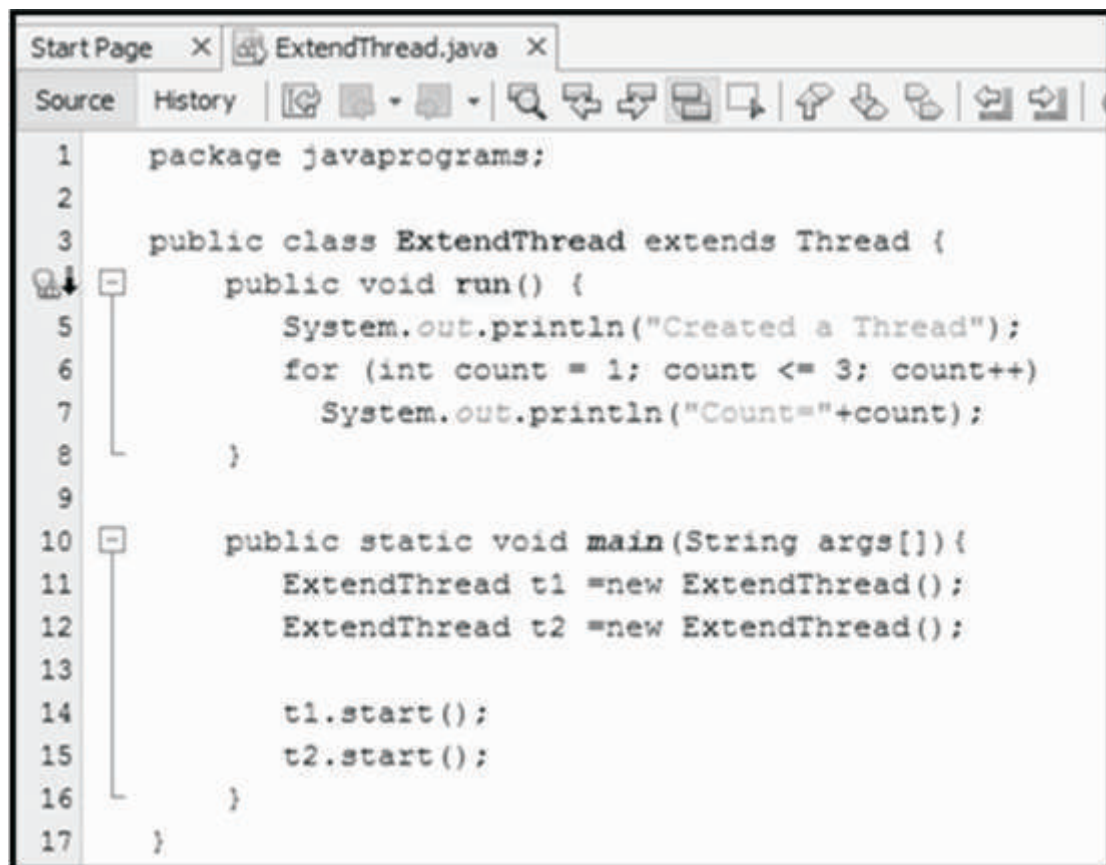
Figure 3.12(d): The ExtendThread Demo Program
