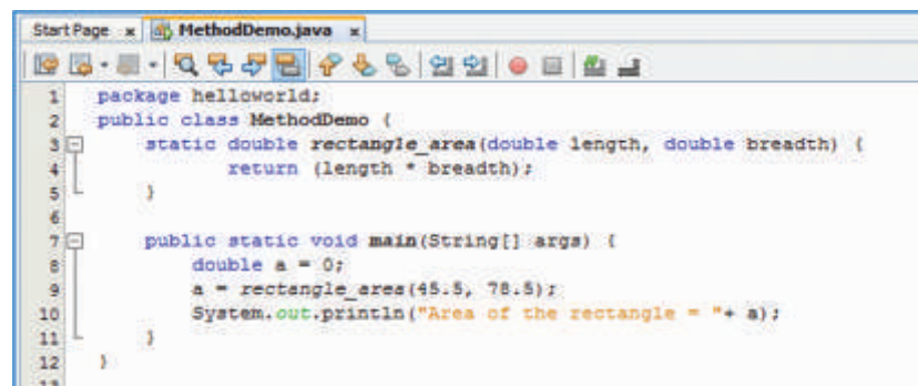
Figure 3.6(a): User Defined Method Demo Program
