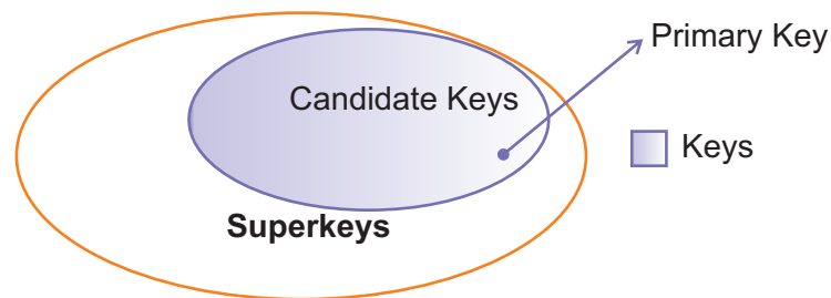
Figure 1.5(c): Superkey, Key, Candidate key and Primary key
