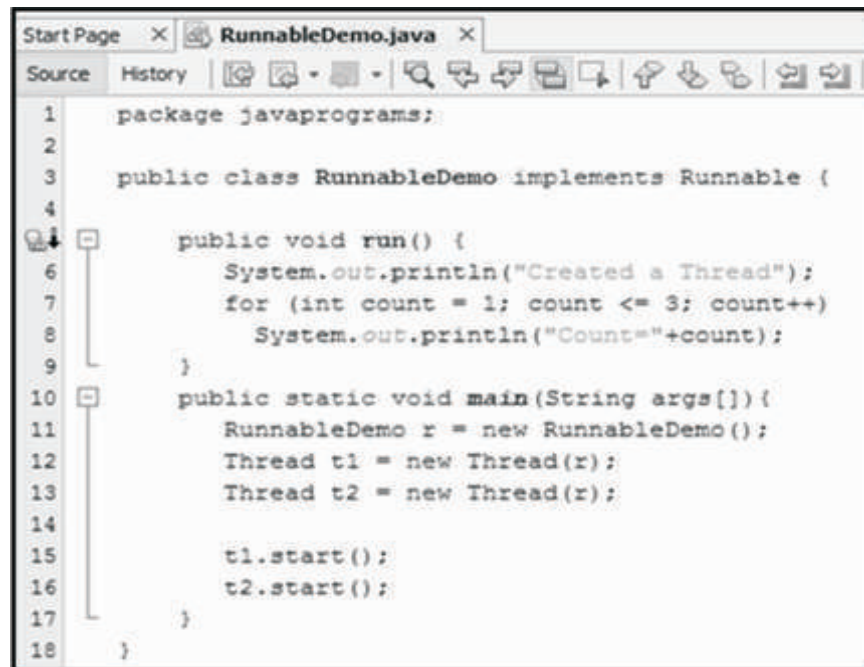
Figure 3.12(f): The RunnableDemo Program
